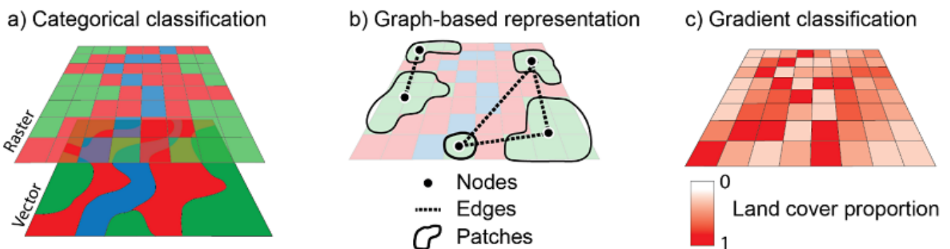
Figure 2. Different data models and landscape conceptualizations for computing landscape metrics: (a) categorical classifications in either raster or vector format, (b) graph-based representations, and (c) gradient, or continuous, classifications where cells represent land cover proportion. Source: author.
