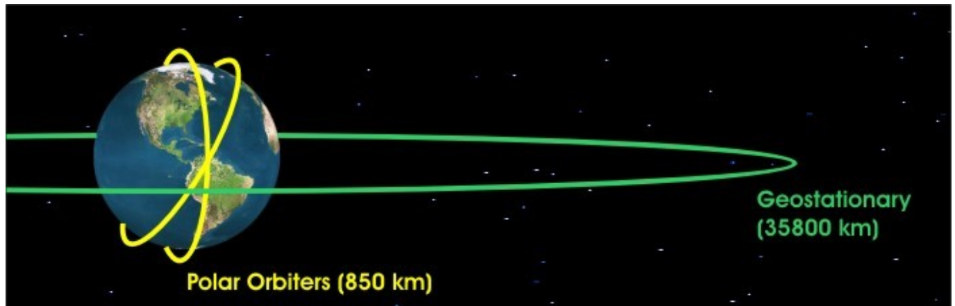
Figure 9. Geostationary versus polar orbiters. Source: David Babb .
