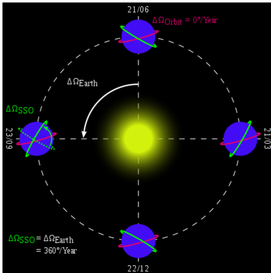
Figure 8: Sun-synchronous orbit. Diagram showing the orientation of a Sun-synchronous orbit (green) at four points in the year. A non-Sun-synchronous orbit (magenta) is shown for reference. Source: Wikipedia.
