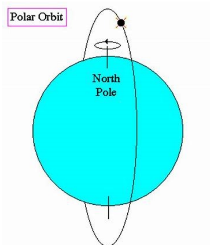
Figure 7: Polar orbit.
